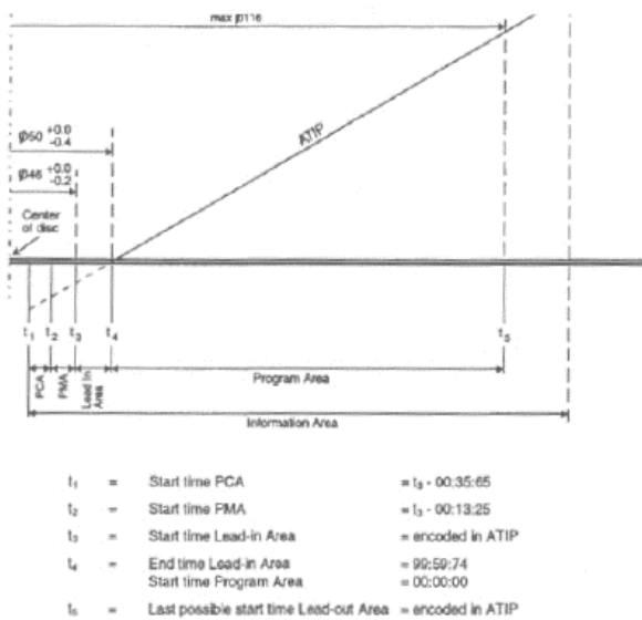
Figure IV - 1 ATIP versus disc diameters
