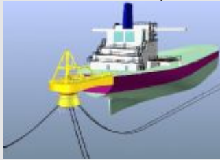
Bluewater Turret System
